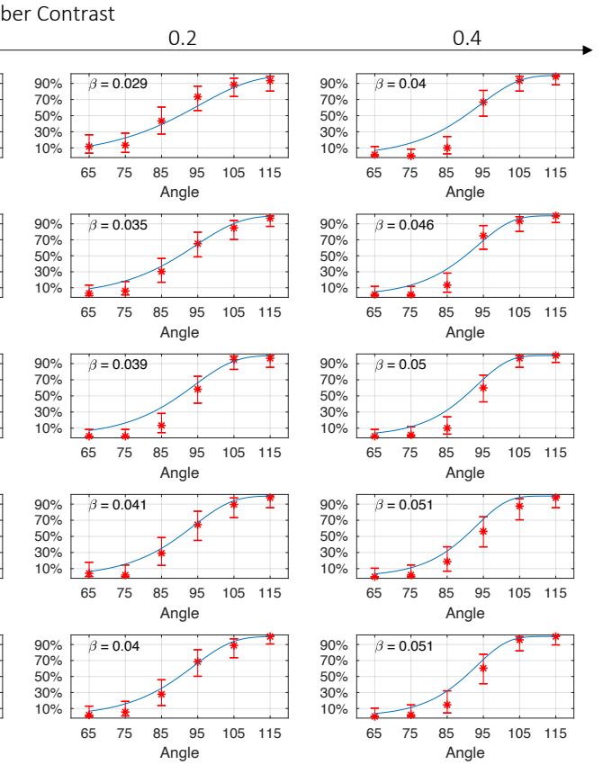
Fig. 4. The red stars are the original data points collected from the 3D shape perception experiment (Section 3). They represent the frequency at which the participants assessed the angle as obtuse under various luminance and contrast conditions. The error bars denote the 99% confidence intervals. The blue curves represent our fitted psychometric model (Section 4). The top-left plot has no data points as it was impossible to see the stimuli at this condition.
